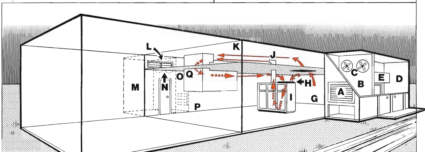
Normal operation—Closed air conditioning system.
