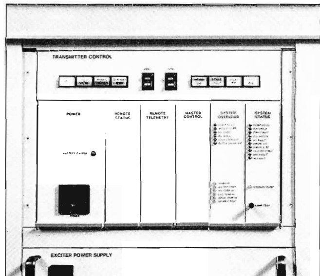
Fig. 4. Transmitter Control and Remote Interface Front Panels
