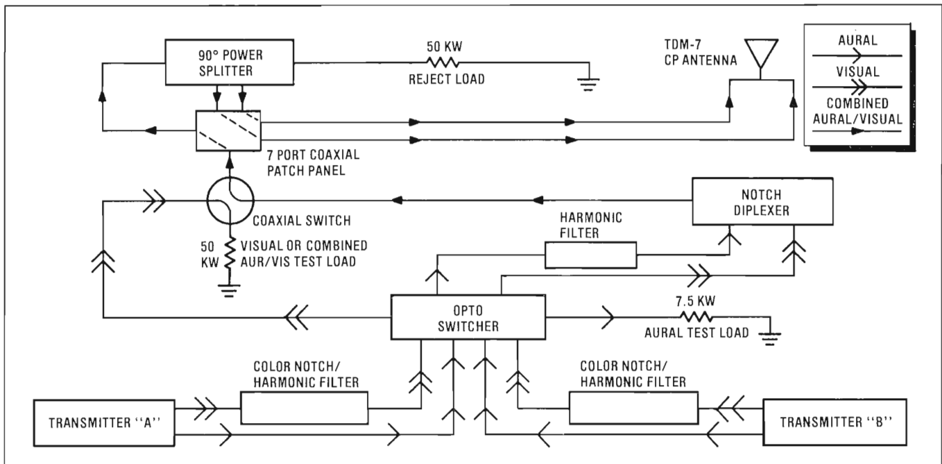
WBRZ-TV RF System Flow Chart.
