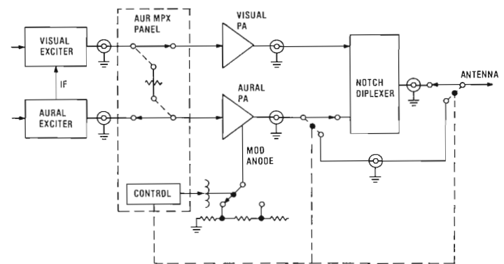
Fig. 6. Aural Power Amplifier Multiplex Switching
