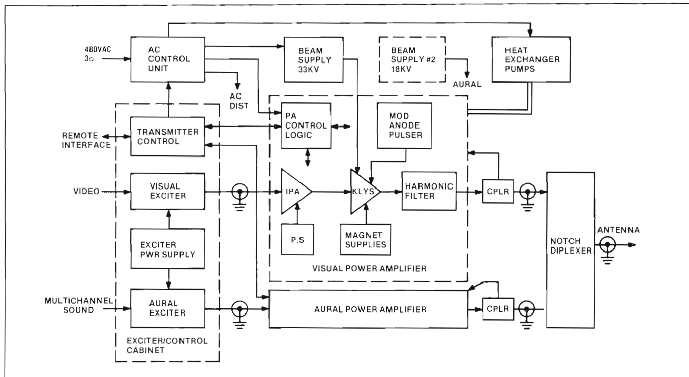
Fig. 3. TTG-100U, Simplified System Diagram
