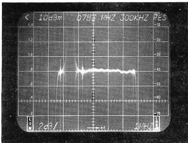
Fig. 9. Frequency Response with Pulsing, 2 dB Division
