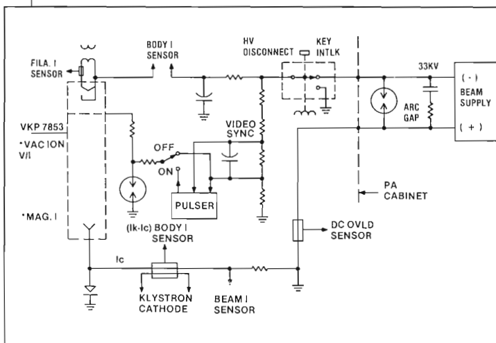
Fig. 5. 100 kW Klystron DC Protection Circuits
